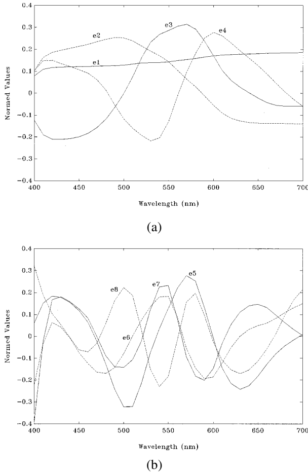
Figure 2. (a) our the first four characteristic vectors (b) our the second four characteristic vectors.
