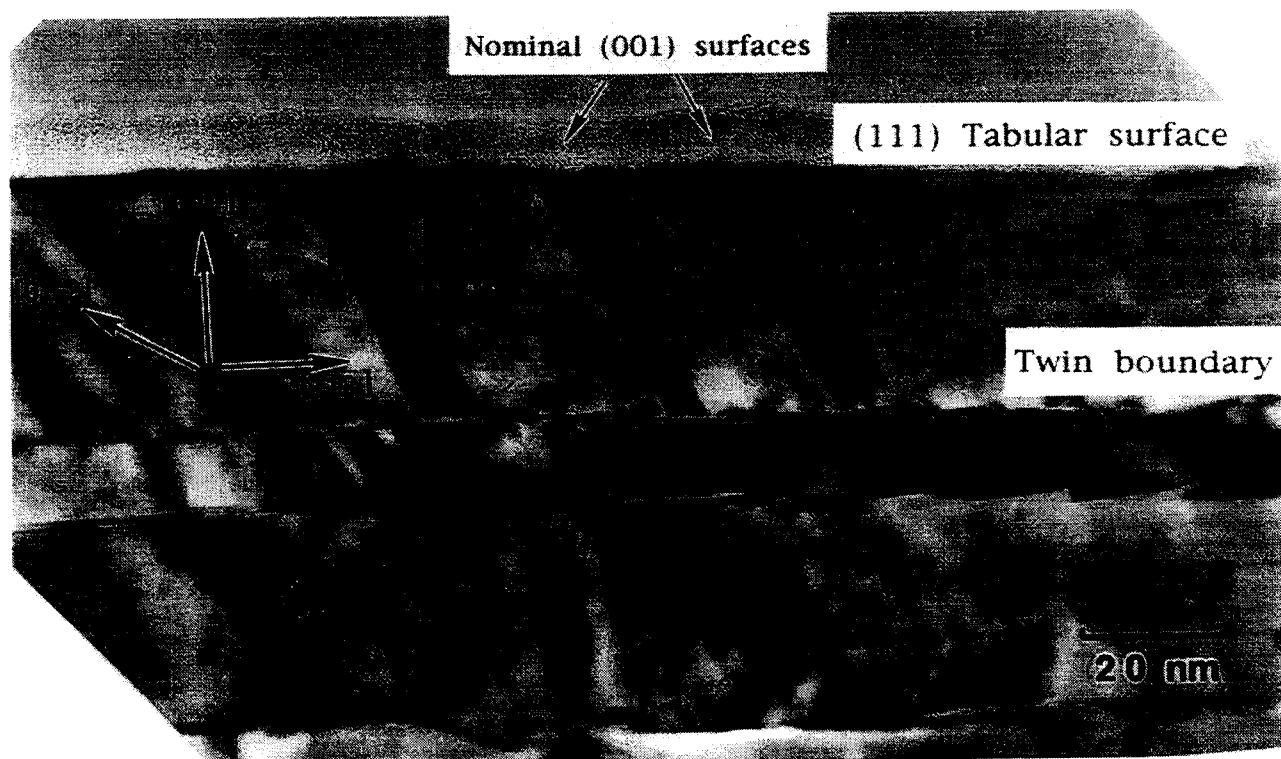
Figure 3. Cross-section image showing three secondary twin bands. Their external surfaces appear to be nominally (001) surfaces.
