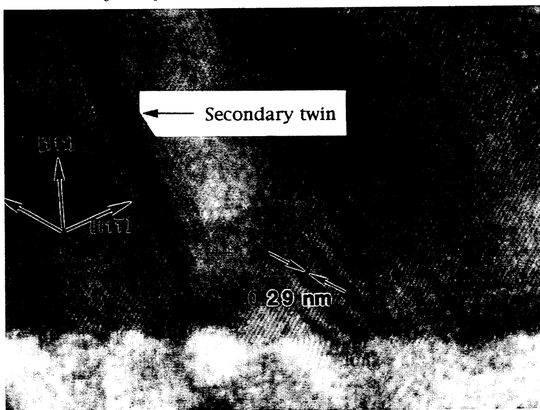
Figure 4. Low-temperature, high-resolution lattice image of a secondary twin band. The secondary twinning occurs across the (111) plane inclined at 70^{\circ} 32' to the primary (111) twin boundary. The (002) spacing, as indicated, is 0.29 nm.
