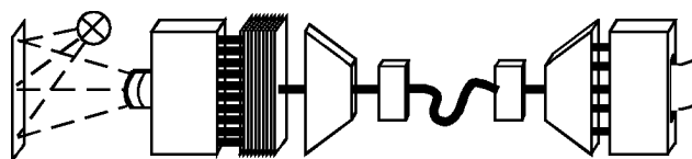
Figure 1. Proposed color reproduction system with multispectral measurement, multispectral encoding and decoding. With the spectral information of each pixel the receiver can optimize the image reproduction.
