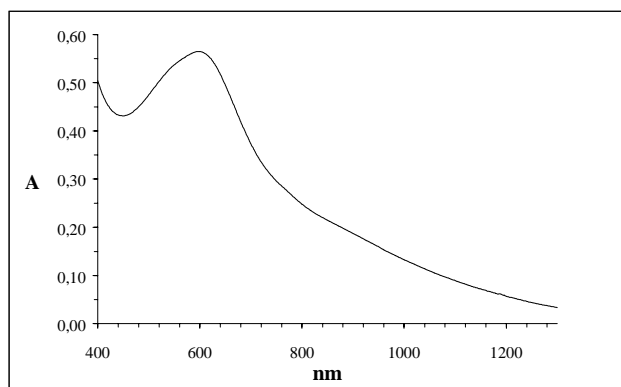
Figure 4: Absorption spectrum of oxidized C.I. Solubilized Sulfur Black 1, 2-ethyl hexylammonium salt in ethanol (54,7 mg/l)
