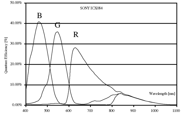
Figure 1. Quantum Efficiency vs. Wavelength
