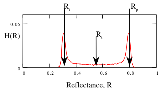
Figure 1: Histogram of 65 LPI AM halftone printed by offset lithography, measured at 5 mm field of view (FOV)
