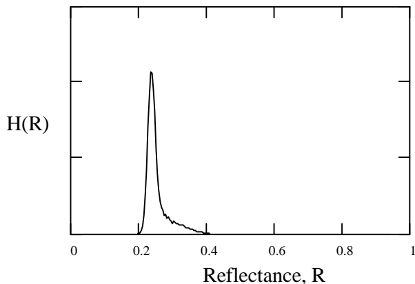
Figure 4. Histograms at 5mm FOV of error diffusion dot pattern printed by thermal ink jet at 300 dpi at a nominal F = 0.05 .
