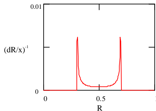
Figure 6: The histogram modeled by equation (2) for the edge in Figure (5).
