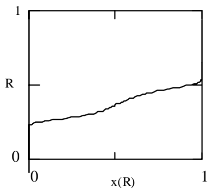
Figure 11: Reflectance as a function of the integral function of the histogram data in Figure 3.
