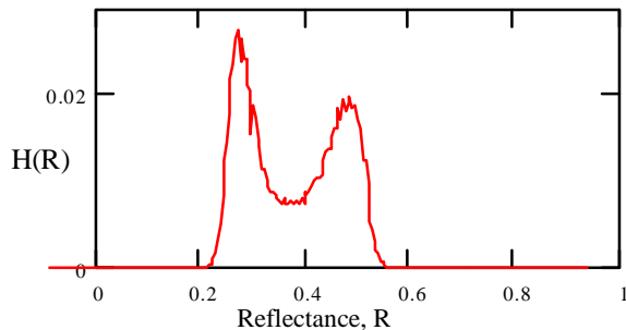
Figure 3. Histograms at 5mm FOV of error diffusion dot pattern printed by thermal ink jet at 300 dpi at a nominal F = 0.5 .
