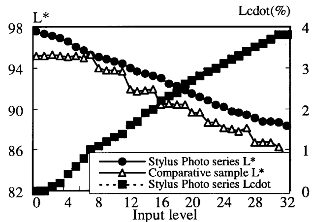
Figure 6: The result of gradation control in highlight area
