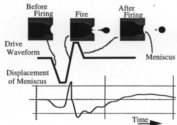
Figure 2: Meniscus control system
