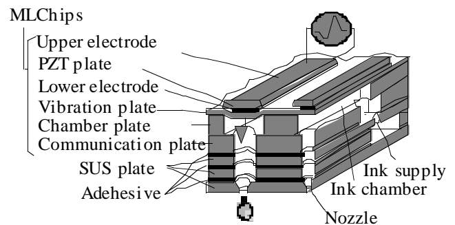
Figure 1: The composition of MLChips type head
