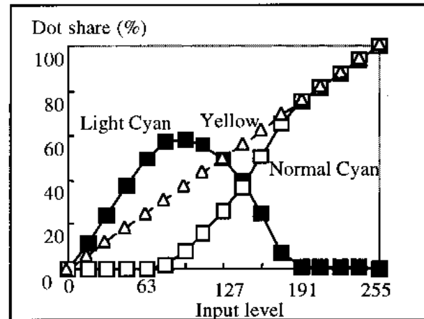
Figure 3: The image of relation between input level and dot share (%)
