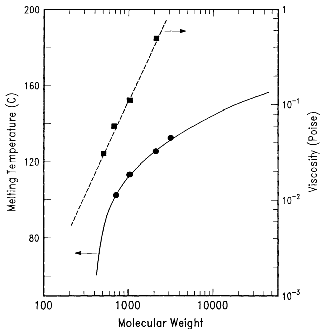
Figure 5. Melting temperature and melt viscosity of PE wax as a function of molecular weight.
