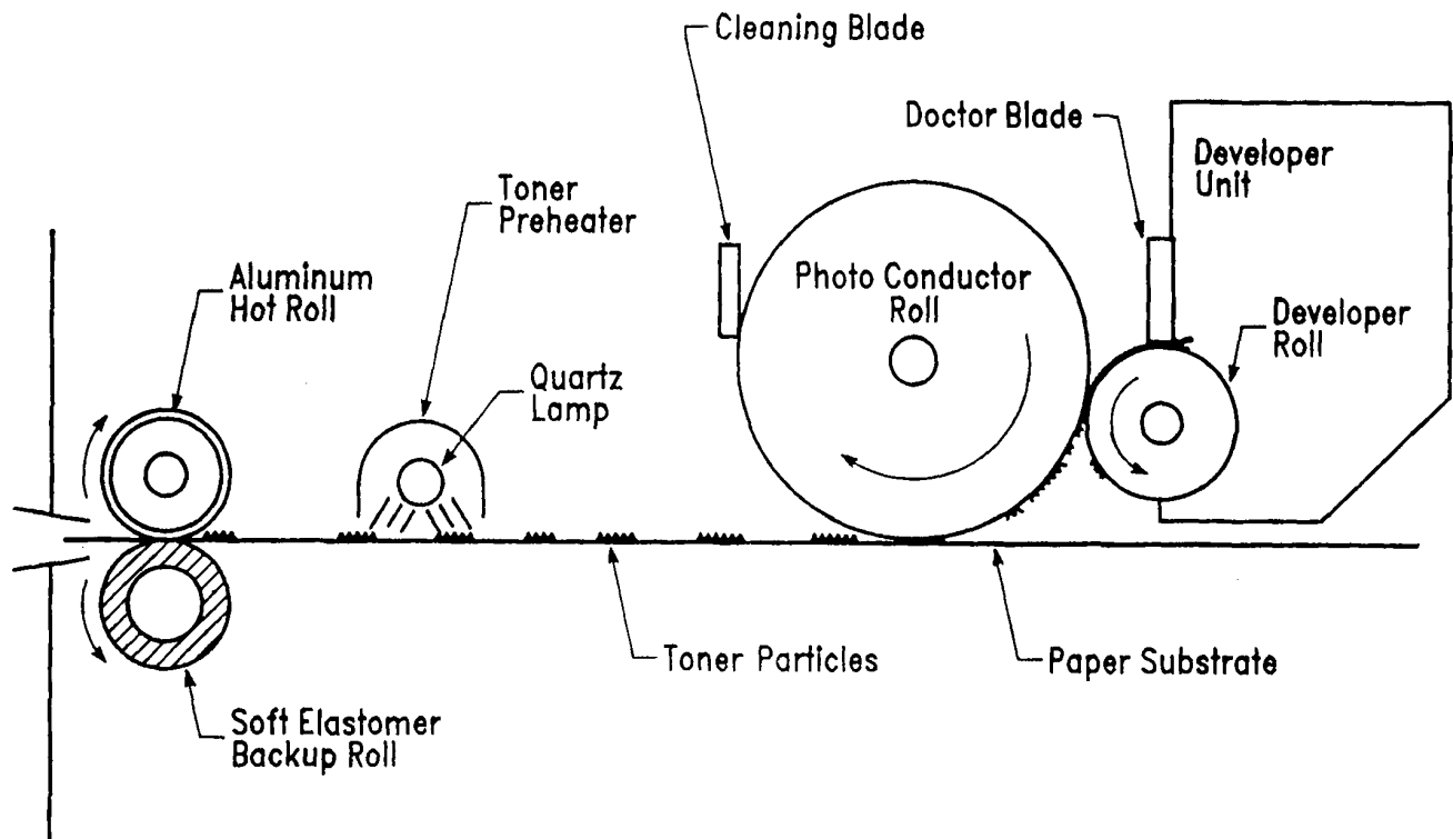
Figure 15. Schematic of the printer robot apparatus used in functional testing of the wax-containing toners.
