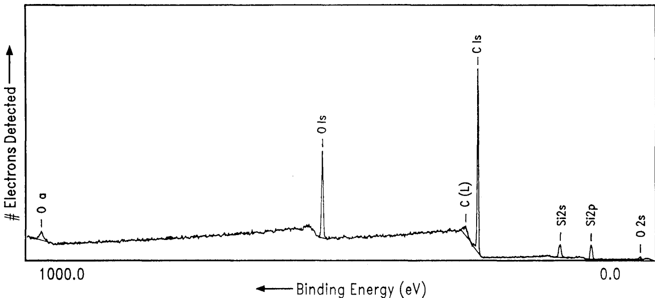
Figure 13. XPS spectrum of a typical toner surface showing the elemental composition.
