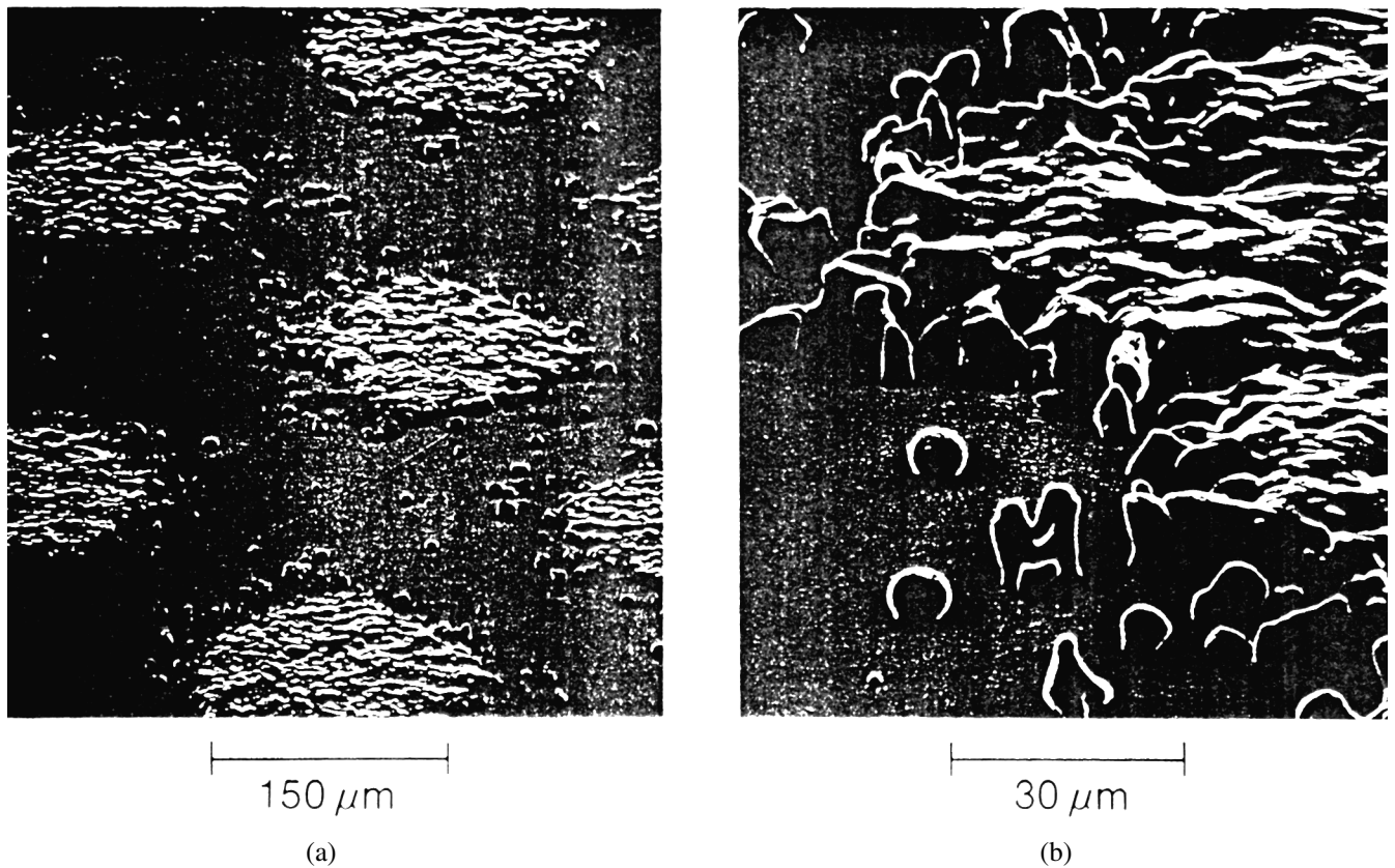
Figure 10. Scanning electron micrographs of toner fused on plastic showing (a) toner scattered around pels and (b) the roughening effect of toner adhesion to the fuser roll.
