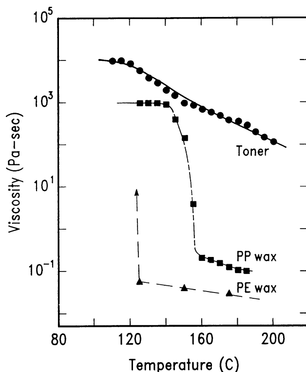
Figure 6. Viscosity of toner compared with typical PP and PE wax as a function of temperature.
