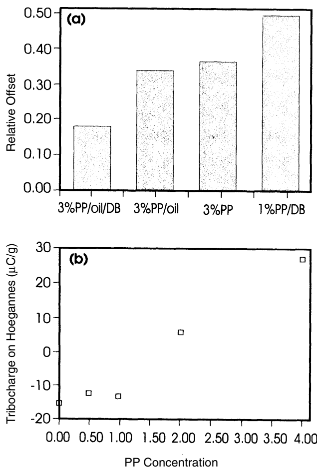
Figure 16. (a) The toner offset for various combinations of PP wax, PDMS oil, and Krayton-G (DB) and (b) the toner charge as a function of PP wax concentration.
