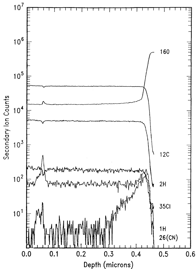
Figure 14. Depth profile of a toner-contaminated fuser roll showing the elemental composition as a function of depth.
