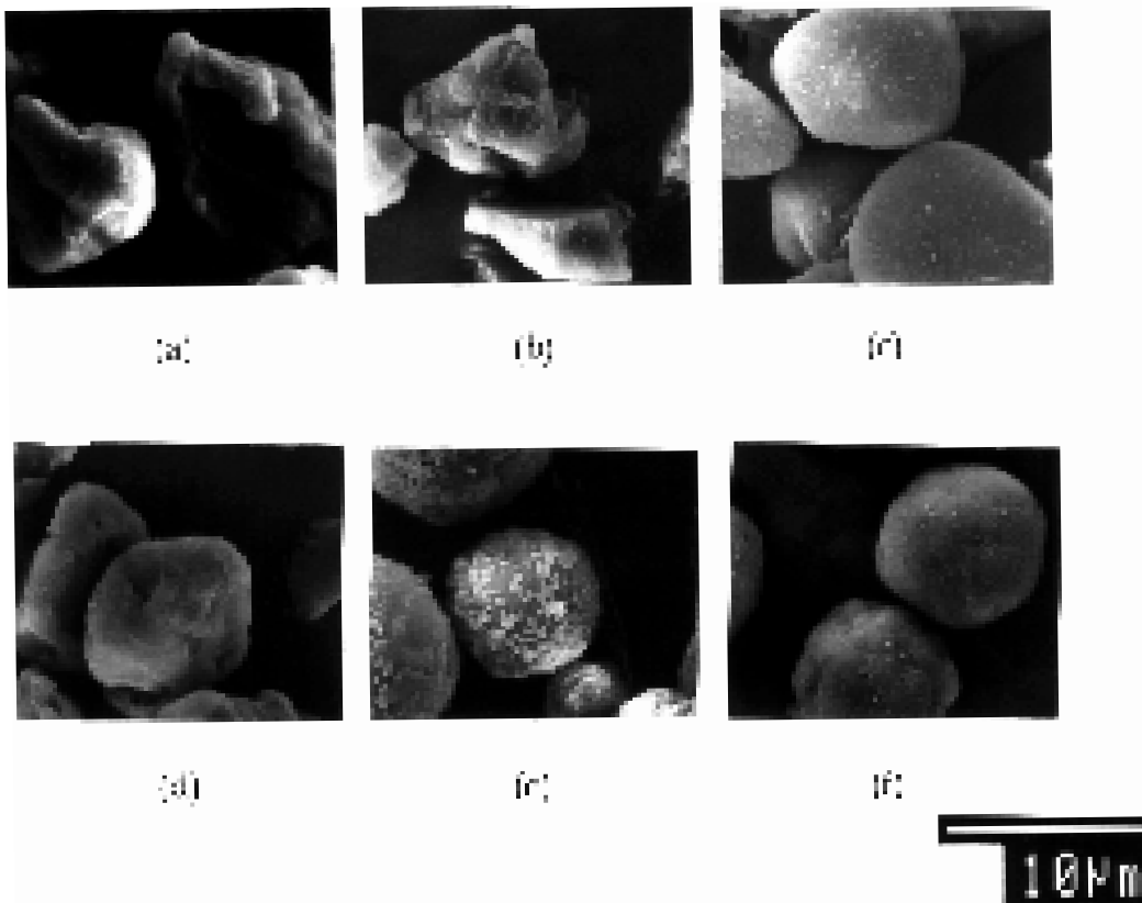
Figure 2. Scanning electron micrographs of the sample toners. (a) IR-U, (b) IR-F, (c) QS-U, (d) QS-F, (e) SP-U, and (f) SP-F.
