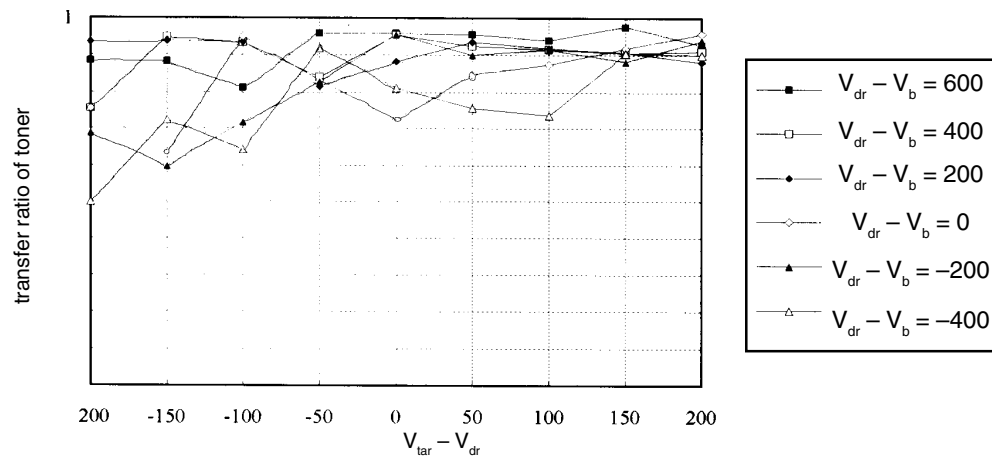
Figure 8. Transfer ratio under different dc bias voltages.
