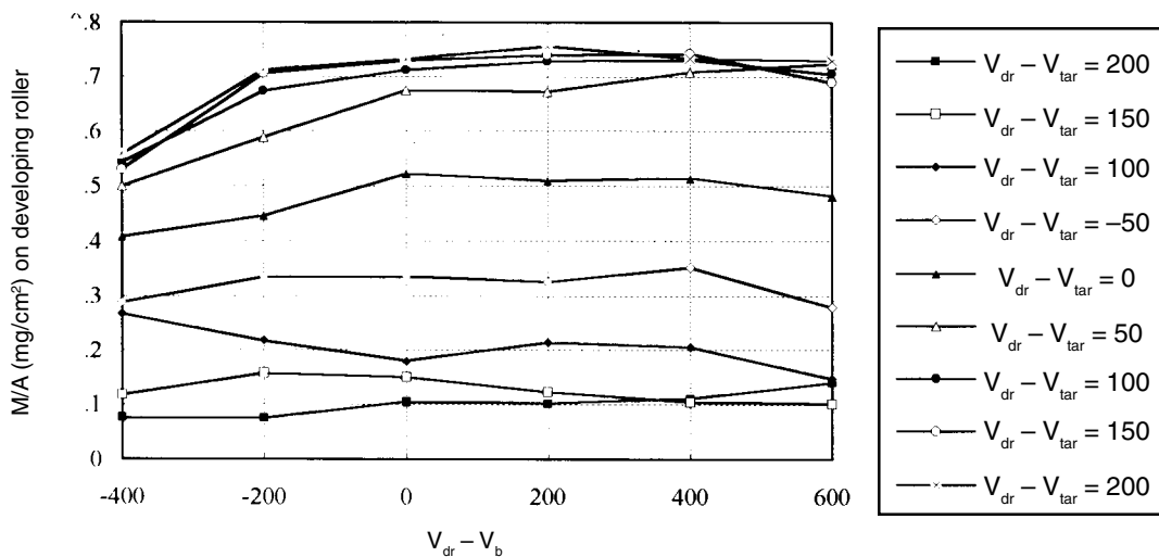
Figure 3. M/A on developing roller.
