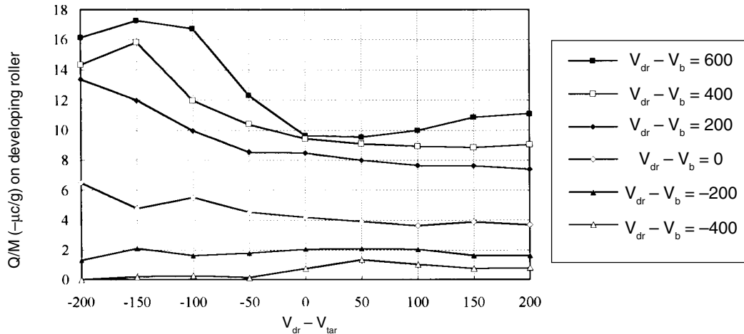
Figure 6. Q/M on developing roller.
