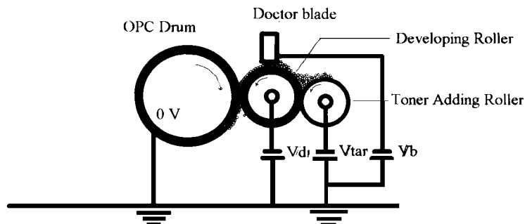
Figure 1. Schematic of the experimental development system.
