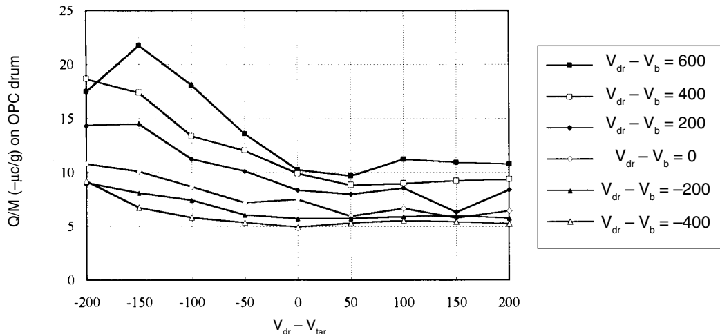
Figure 7. Q/M on OPC drum.
