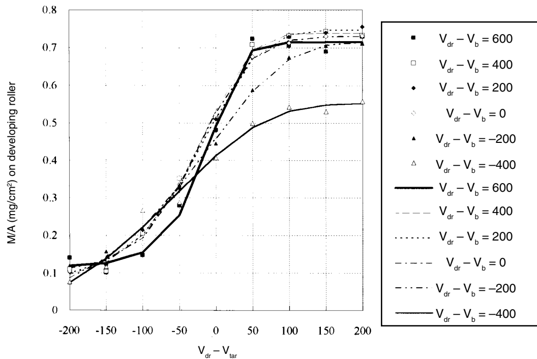
Figure 2. M/A on developing roller.
