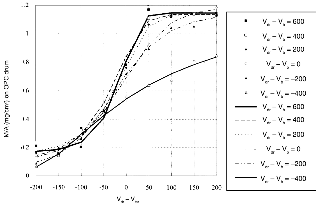
Figure 4. M/A on OPC drum.
