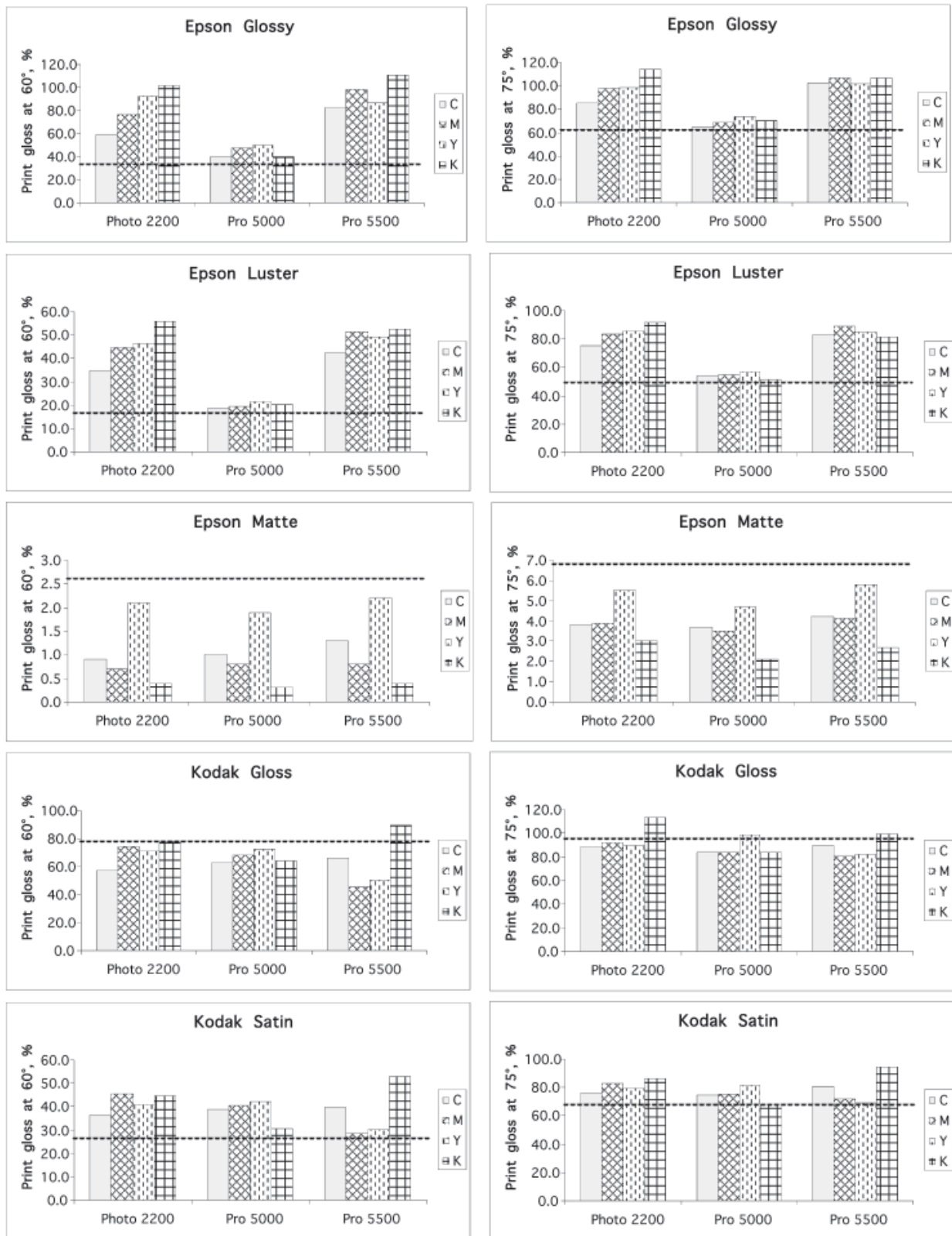
Figure 2. Comparisons of print gloss at 60° (left) and 75° (right) between three printers for all five papers, with dotted line indicating paper gloss value. (Print gloss lower than the paper gloss results in negative delta gloss).
