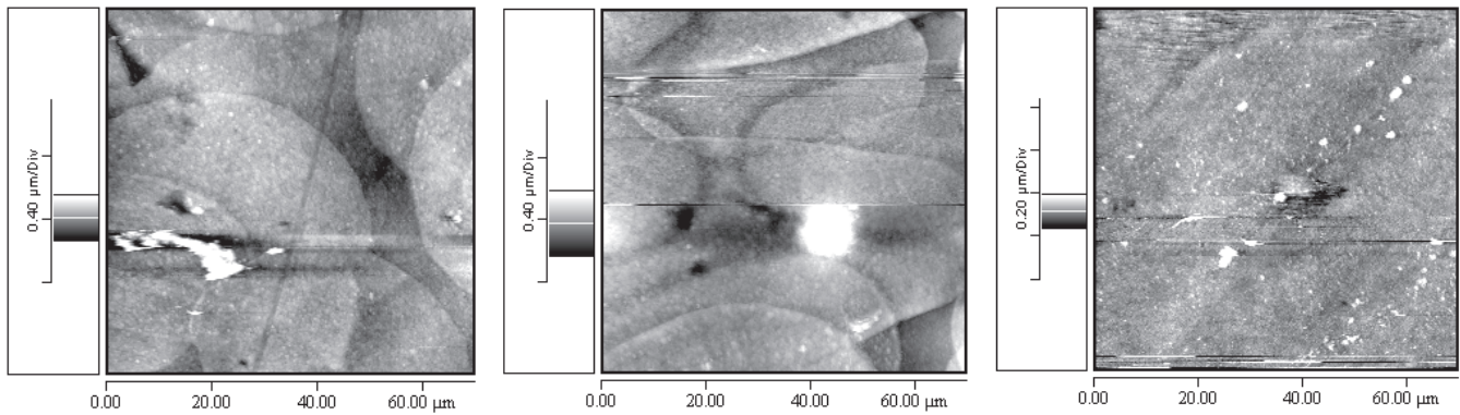
Figure 3. AFM images of black ink film topography on Epson Glossy paper printed by: Pro 5500 printer (left), Photo 2200 printer (center), and Pro 5000 printer (right).
