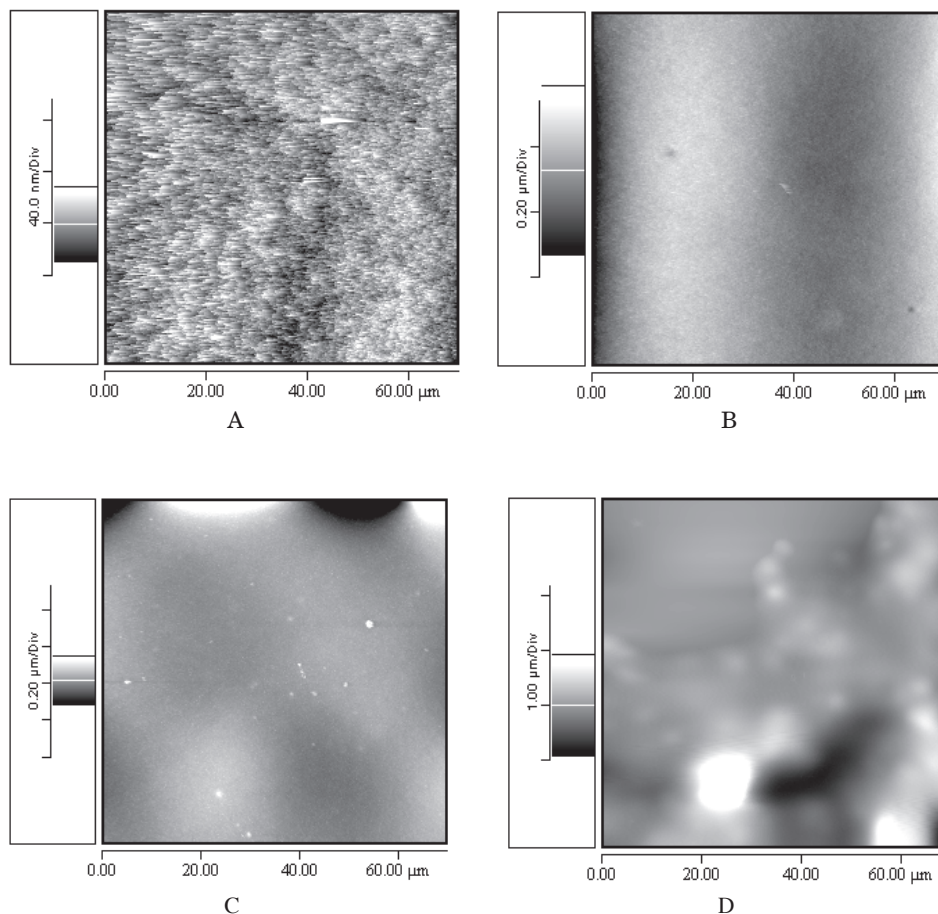
Figure 1. AFM images of paper topography: Epson Glossy (A-upper left), Epson Luster (B-upper right), Kodak Gloss (C-lower left), and Kodak Satin (D-lower right).
